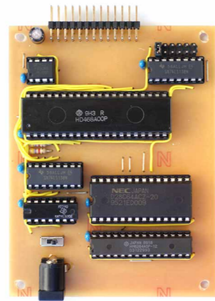
6800 CPU Board (Prototype)
