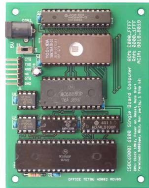
SBC6800 Single Board Computer
